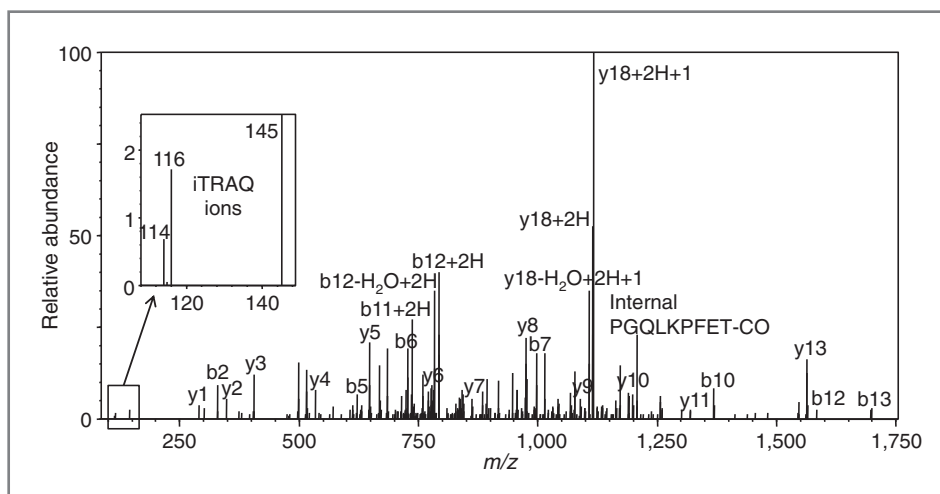
Figure 2. Positive ion nano-electrospray Q/D and collision-induced dissociation product ion tandem mass spectrum of peptide ALPGQLKPFETLLSQNQGK from GSTP1 protein which was upregulated in the cytosolic/membrane fraction. The triply protonated precursor ion was observed at m/z 853.831 corresponding to an uncharged mass of 2558.47 u ( \Delta M 2.2 ppm). Note the iTRAQ reporter ions of m/z 114, m/z 116 and m/z 145 that were used for the determination of relative protein expression in PrE cells treated with lycopene or placebo beadslets.
