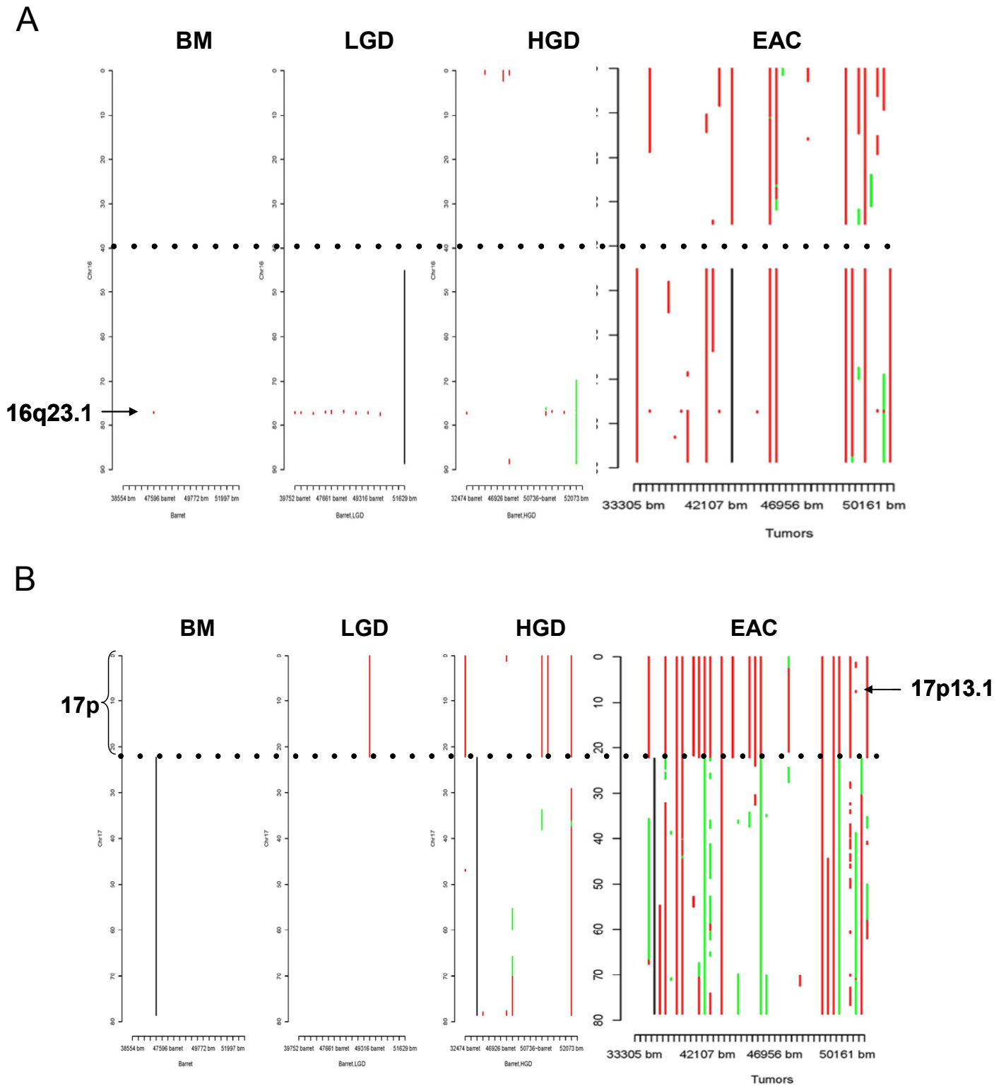
Supplementary Fig. 1. Distribution of aberrations at chromosomes 16 (A) and 17 (B) in different stages from BM to EAC. X axis denotes samples, Y axis denotes chromosome position in Mb. Red: loss, Green: amplification, Black: aberrations ambiguous, Dotted black: centromere position.
